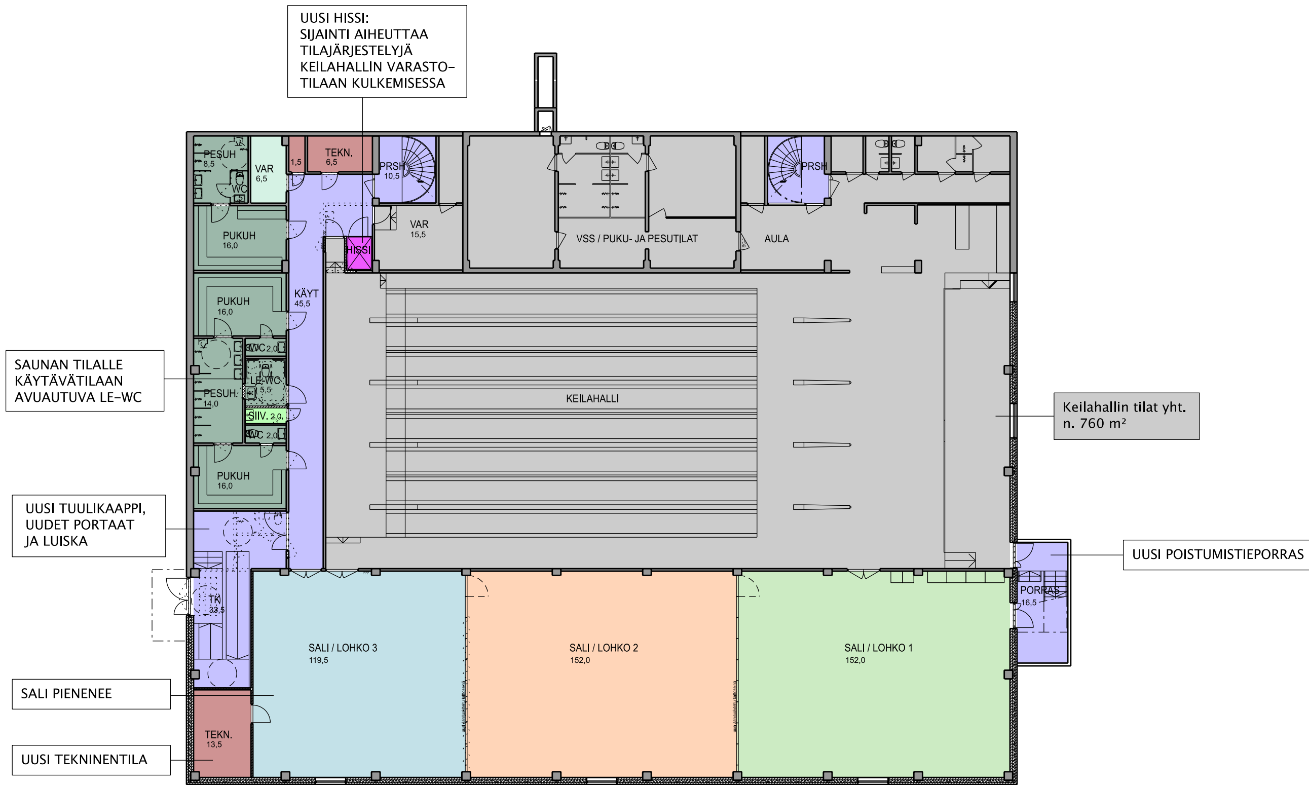
K kerros (=KEILAHALLI +68.723)
